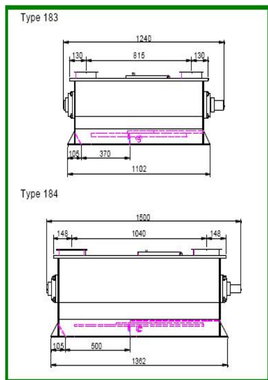
Figure 1: 尺寸
